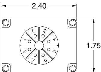
Series 5400 Relay Dimensions
